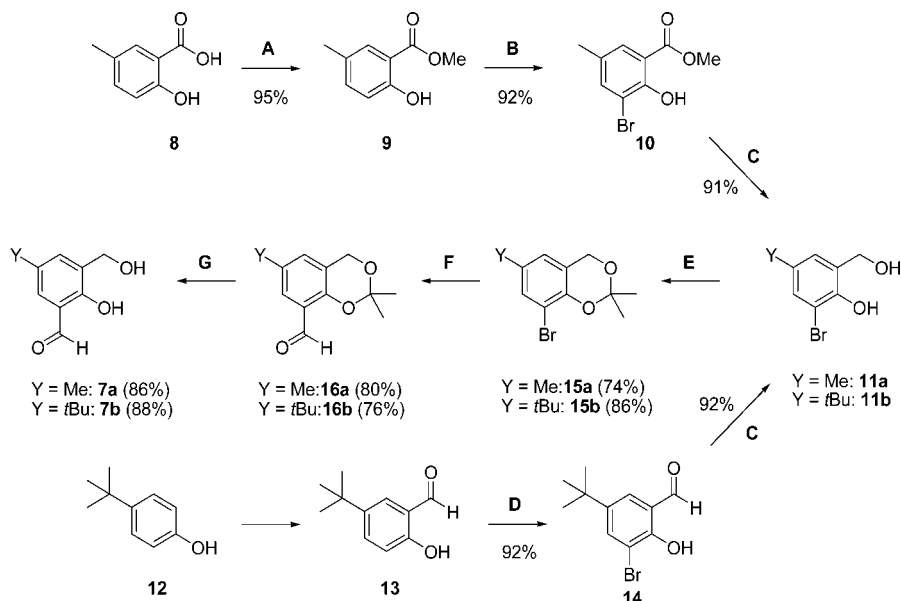
Scheme 1. Synthesis of the 6-Formyl-4-alkylsalicyl Alcohols 7a and 7b a
